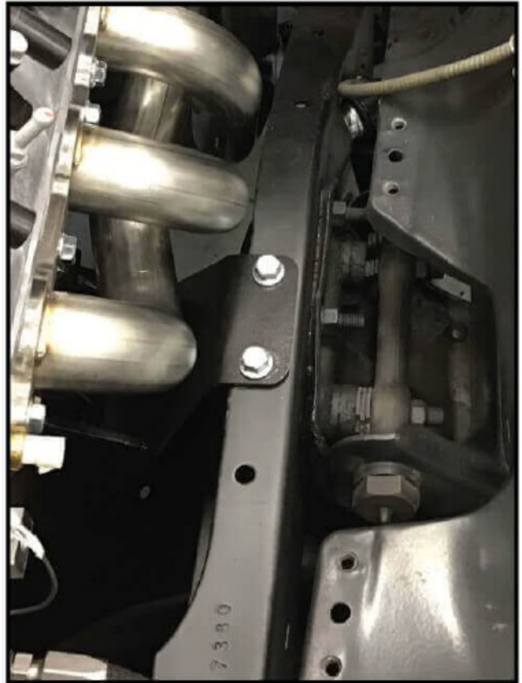
Narrow Frame-rail
